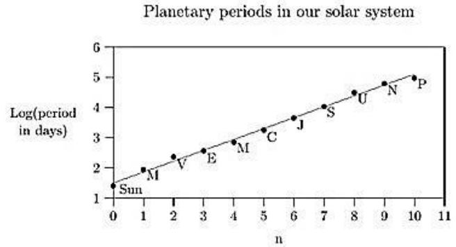
Figure 8 Bode's Law for the Sun and Its Planets
