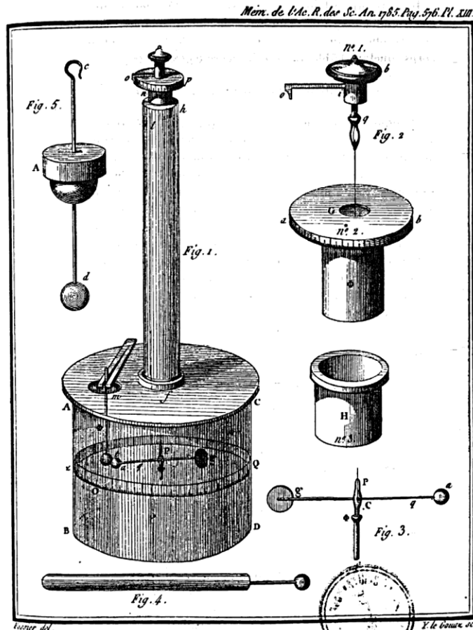
Figure 3 Coulomb's Torsion Balance
