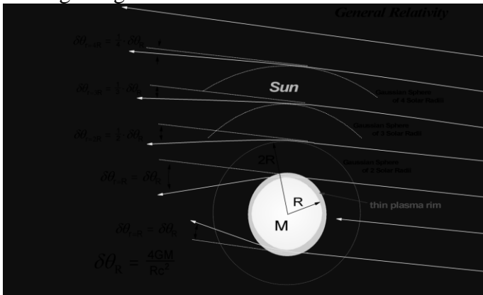
Figure 6 General Relativity Predicted Bending of Starlight by the Sun [16, 17]
