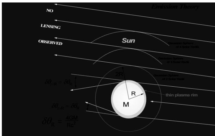
Figure 7 Observed Bending of Starlight by the Sun [16, 17].
