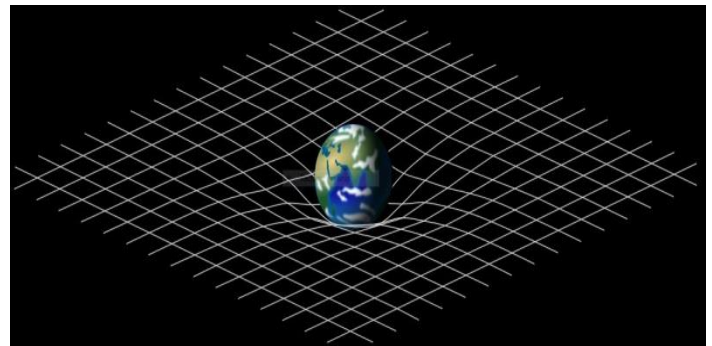
Figure 4 Fabric of Einstein's Spacetime
