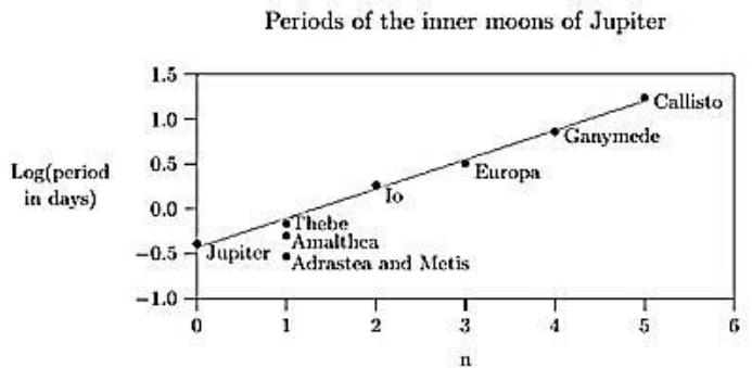
Figure 9 Bode's Law for Jupiter and Its Moons
