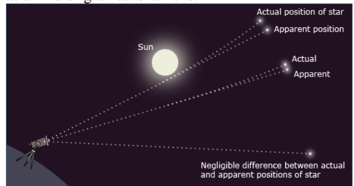
Figure 5 Bending of Starlight Passing Near the Sun
