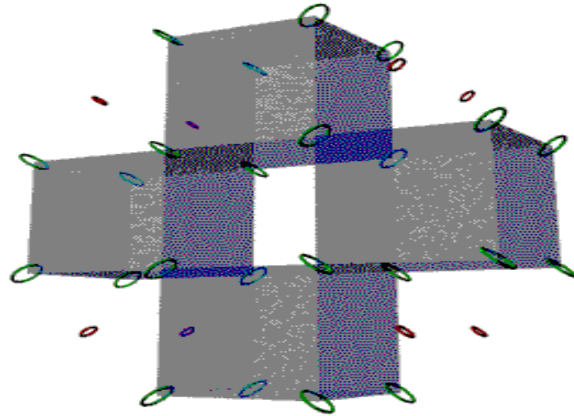
Figure 7. Cyclobutane C_4H_8
