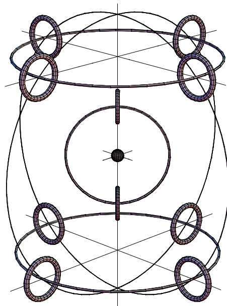
Figure 2. Neon-20 Atom
